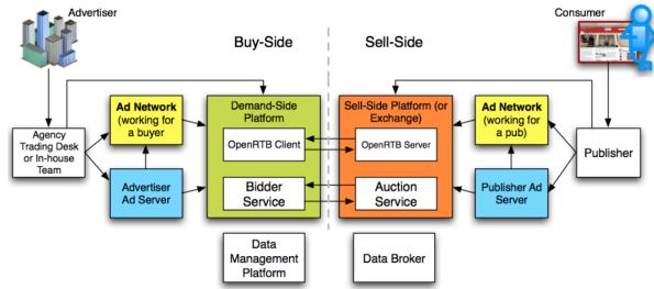
Figure 1: High-level communication between parties in the Open RTB Ecosystem [24] (courtesy: Interactive Advertising Bureau).
